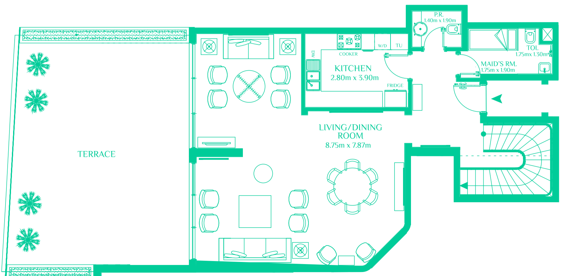
Duplex-B Lower Level 163.2 sqm
